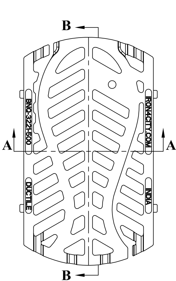
PLAN VIEW
